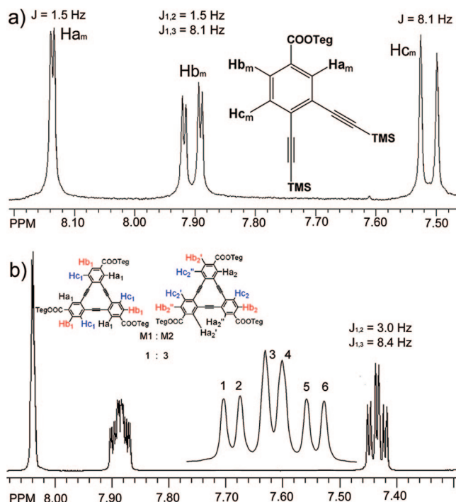
Figure 3. ^1\text{H} NMR spectrum of precursor and macrocycle isomers. (a) Aromatic region of the ^1\text{H} NMR spectrum of the precursor. (b) Aromatic region of the ^1\text{H} NMR spectrum of macrocycle isomers.
