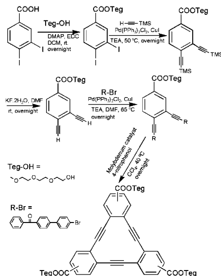
Scheme 1. Synthetic Route of Macrocycle Isomers
