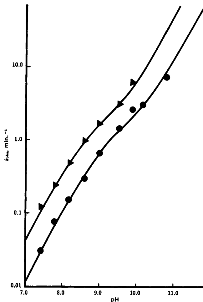
Figure 4 —Log k_{\text{obs}} versus pH profile for the closure of III at 25° (●) and 37° (▲) ( \mu = 1.0 , with potassium chloride).
