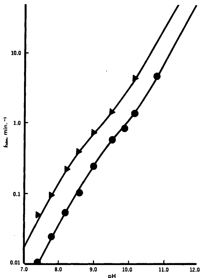
Figure 3 —Log k_{\text{obs}} versus pH profile for the closure of V at 25° (●) and 37° (▲) ( \mu = 1.0 , with potassium chloride).
