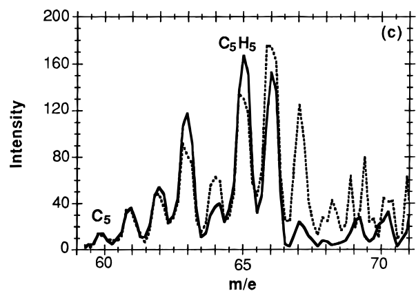
Figure 4. High-resolution mass spectra of n = 3, 4, 5 regions, for products from ethane at 1068 °C and 85 Torr (full traces) compared with equimolar mixture of CD_4 and C_2H_6 at 1068 °C and total 85 Torr (dashed traces, normalized to full traces at the C_n peak). Note variation with n of ordinate scale.
