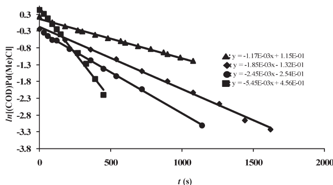
Figure 5. Pseudo-first-order kinetic plots for the substitution reactions of (\text{COD})\text{Pd}(\text{Me})\text{Cl} with various \alpha -aminoaldehydes at 0 °C in \text{CDCl}_3 ( \blacklozenge , L6a ; \blacksquare , L6b ; \bullet , L7a ; \blacktriangle , L7c ).
