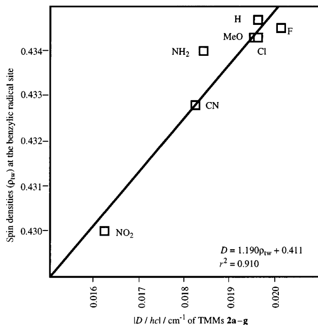
Fig. 3 AM1/AUHF-calculated spin densities ( \rho_{tw} ) at the benzylic radical site versus |D|/hc/\text{cm}^{-1} values of the TMMs 2a–g
