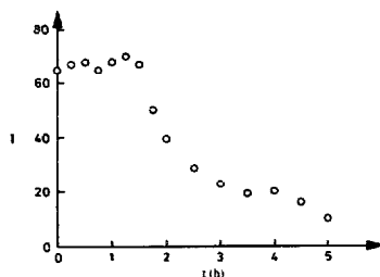
Fig. 2. 1 H NMR decay profile for the reaction of 1 with TsCl. I = [I(Me)/I(CH_2Cl_2)] \times 100 .
