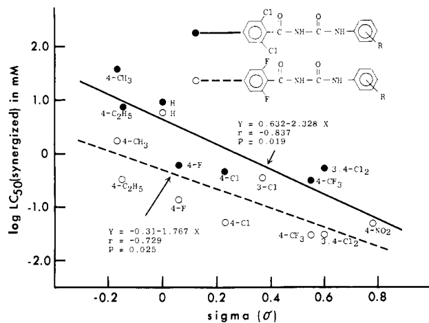
Figure 1. Correlation of insecticidal activity and Hammett's \sigma constant for substituted 1-phenyl-3-(2,6-dichlorobenzoyl)- and 1-phenyl-3-(2,6-difluorobenzoyl)-ureas.
