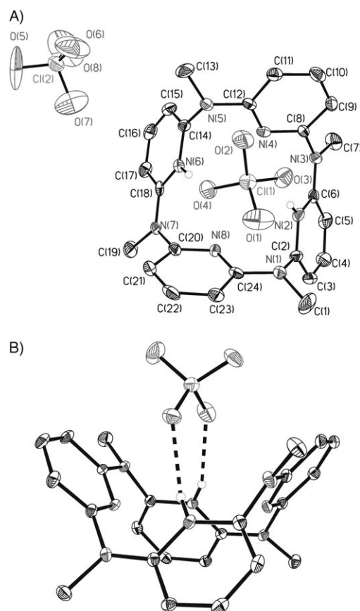
Figure 6. Molecular structure of diprotonated methylazacalix[4]pyridine [H_2\mathbf{10}]2 ClO_4 : A) top view and B) side view (one ClO_4^- omitted for clarity). Selected bond lengths [Å]: C(6)–N(3) 1.319, N(3)–C(8) 1.427, C(12)–N(5) 1.380, N(5)–C(14) 1.397, C(18)–N(7) 1.373, N(7)–C(20) 1.418, C(24)–N(1) 1.385, N(1)–C(2) 1.395; selected interatomic distances [Å]: N(2)⋯N(4) 2.987, N(2)⋯N(8) 3.032, N(6)⋯N(4) 3.026, N(6)⋯N(8) 3.040, N(6)⋯O(4) 2.916, N(2)⋯O(3) 3.033, C(10)⋯C(22) 8.283.
