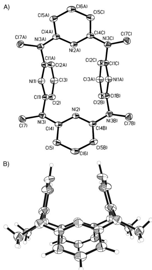
Figure 1. Crystal structure of methylazacalix[4]pyridine 10 : A) top view and B) side view. Selected bond lengths [Å]: C(1)–N(3) 1.436, C(4)–N(3) 1.389; selected interatomic distances [Å]: C(3)···C(3A) 3.422, N(1)···N(1A) 4.620, N(2)···N(2A) 4.835, C(6)···C(6A) 9.063, N(1)···N(2) 3.353.
