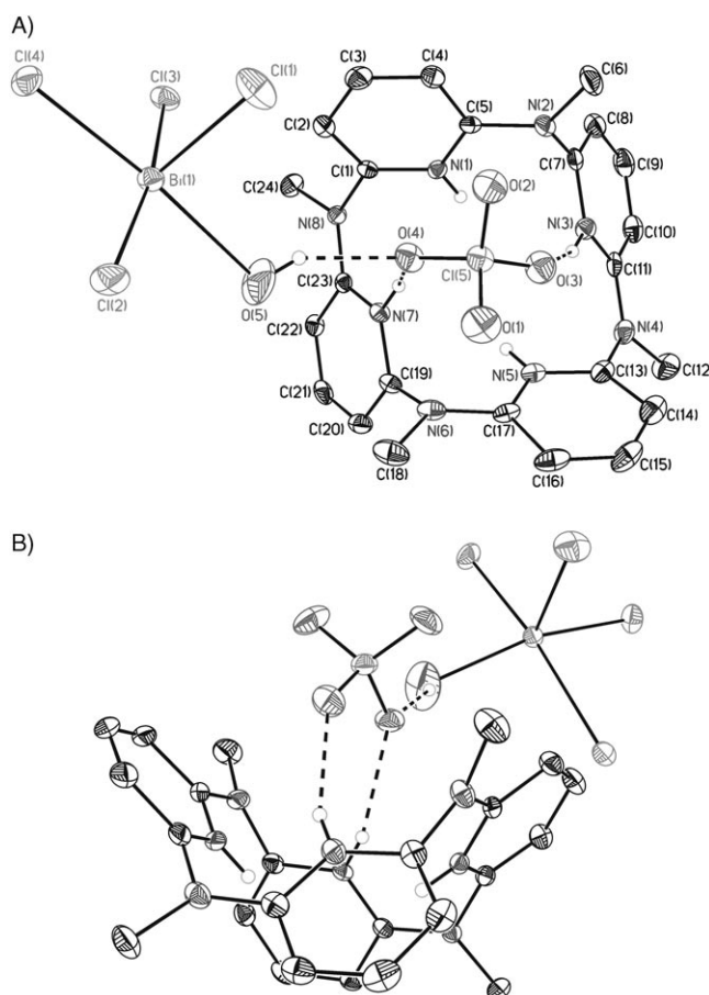
Figure 7. Molecular structure of triprotonated methylazacalix[4]pyridine [H_3\mathbf{10}] ClO_4 \cdot OH \cdot BiCl_4 : A) top view and B) side view. Selected bond lengths [Å]: C(5)–N(2) 1.387, N(2)–C(7) 1.397, C(11)–N(4) 1.348, N(4)–C(13) 1.420, C(17)–N(6) 1.390, N(6)–C(19) 1.399, C(23)–N(8) 1.343, N(8)–C(1) 1.436; selected interatomic distances [Å]: N(1)⋯N(7) 2.955, N(1)⋯N(3) 3.063, N(3)⋯N(5) 2.964, N(3)⋯O(3) 3.086, N(7)⋯O(4) 2.965, O(4)⋯O(5) 2.875, O(5)⋯Bi(1) 2.710, C(3)⋯C(15) 8.417.
