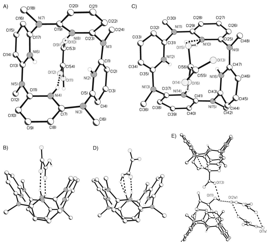
Figure 8. Molecular structure of 10 ·HO 2 CCO 2 H·H 2 O: A) top view and B) side view of the complex of the triprotonated methylazacalix[4]pyridine with a planar HO 2 CCO 2 − . C) Top view and D) side view of the triprotonated methylazacalix[4]pyridine with a twisted HO 2 CCO 2 − . E) Side view of a heterodimeric structure. Selected bond lengths [Å]: C(5)–N(3) 1.410, N(3)–C(7) 1.379, C(11)–N(5) 1.352, N(5)–C(13) 1.332, C(17)–N(7) 1.400, N(7)–C(19) 1.304, C(23)–N(1) 1.427, N(1)–C(1) 1.303, C(47)–N(9) 1.418, N(9)–C(25) 1.406, C(29)–N(11) 1.378, N(11)–C(31) 1.441, C(35)–N(13) 1.435, N(13)–C(37) 1.430, C(41)–N(15) 1.308, N(15)–C(43) 1.446; selected interatomic distances [Å]: N(4)···N(6) 2.995, N(8)···N(2) 3.050, N(8)···O(10) 2.679, N(4)···O(12) 2.704, C(3)···C(15) 7.387, N(12)···N(14) 2.997, N(16)···N(10) 2.953, N(14)···O(16) 2.734, N(10)···O(15) 2.921, C(33)···C(45) 7.413, O(11)···O(13) 2.572, O(11)···O(2W) 2.571.
