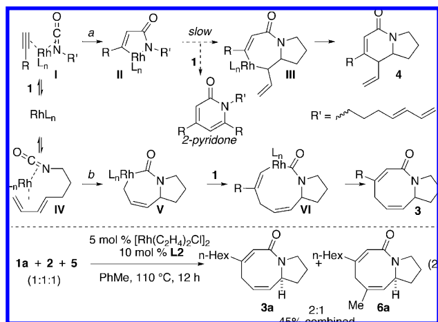
Scheme 1. Proposed Mechanism
