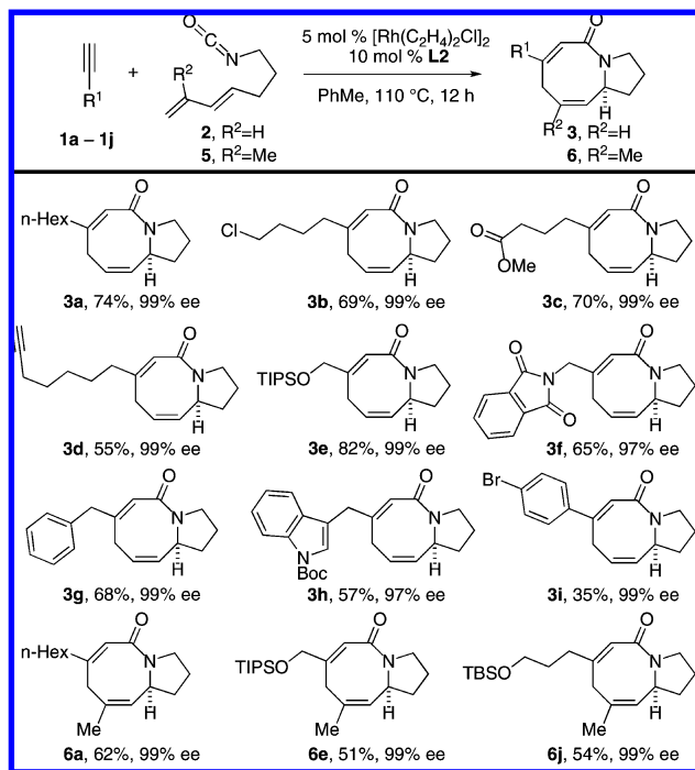
Chart 1. Enantioselective Synthesis of [6.3.0] Bicyclic Azocines
