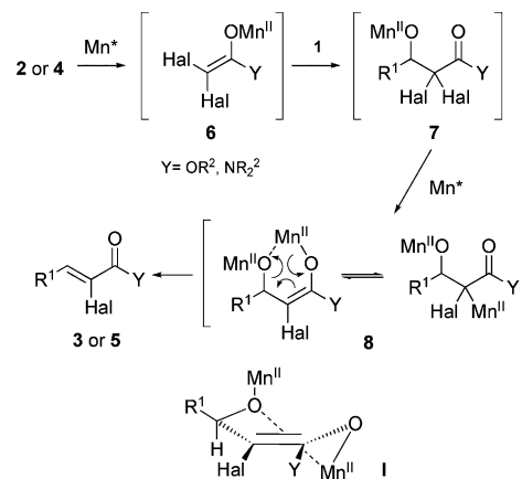
Scheme 1 Proposed mechanism.
