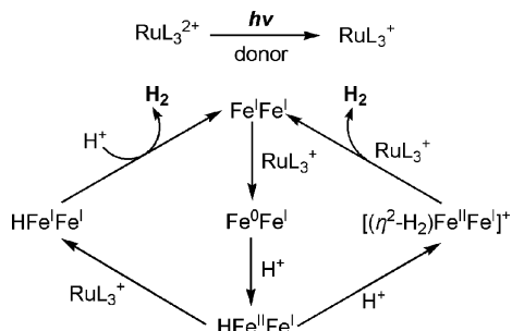
Scheme 2. The Proposed Photochemical Proton Reduction Processes Catalyzed by the Biomimetic [2Fe2S] Complexes
