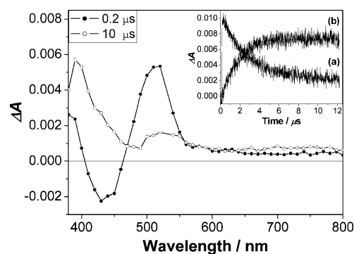
Figure 1. Transient absorption spectra obtained at 0.2 \mu\text{s} and 10 \mu\text{s} following laser flash photolysis of a deoxygenated CH 3 CN solution containing Ru(bpy) 3 2+ (0.03 mM), dtc - (1.0 mM) and 2 (0.2 mM). Inset: kinetic traces at 520 nm (a) and 400 nm (b).
