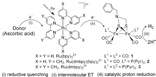
Scheme 1. The Homogeneous Molecular Three-Component System for Photochemical H 2 Generation Catalysed by [FeFe]H 2 ase Active Site Mimics
