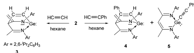
Scheme 3 The reaction of 2 with HC \equiv CH and HC \equiv CPh.
