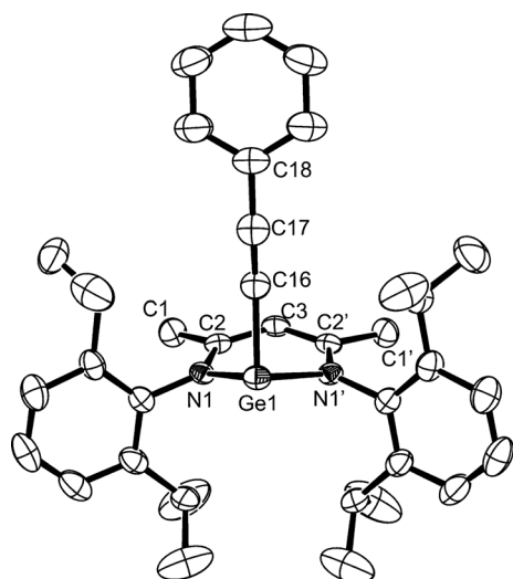
Fig. 3 Molecular structure of 5 . Thermal ellipsoids are drawn at 50% probability level. Hydrogen atoms are omitted for clarity. Selected bond lengths (pm) and angles ( ^{\circ} ): Ge1–C16 197.6(4), Ge1–N1 198.5(2), N1–C2 134.5(3), C2–C3 139.0(3), C16–C17 121.9(5), C16–Ge1–N1 93.35(9), N1'–Ge1–N1 91.3(1), C2–C3–C2' 127.9(3), C17–C16–Ge1 171.0(3), C16–C17–C18 176.6(4). The sum of angles at Ge is 278. Symmetry transformations used to generate equivalent atoms ( ' ): x, -y + 3/2, z .
