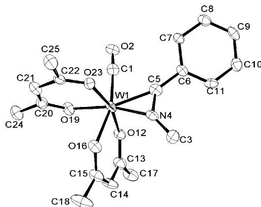
Figure 1. ORTEP diagram of [W(CO)(acac)_2(\eta^2-MeN=CPh)]^+ [OTf]^- ( 2a ). Thermal ellipsoids are drawn with 50% probability. Hydrogen atoms and triflate counterion omitted for clarity.
