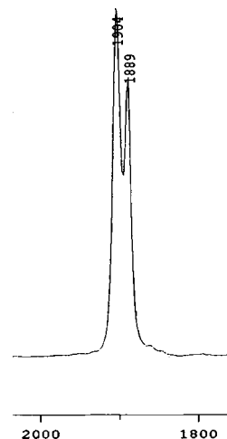
Figure 2. Expanded IR spectrum of W(CO)(acac)_2(\eta^2-MeN=CPh) ( 2a ) in hexanes showing the CO absorption frequency of both diastereomers.
