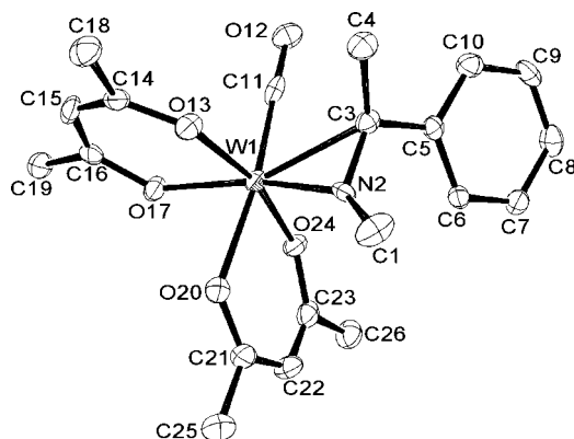
Figure 3. ORTEP diagram of \text{W(CO)}_2(\text{acac})_2(\eta^2\text{-MeN=CHMePh}) ( 4 ). Thermal ellipsoids are drawn with 50% probability. Hydrogen atoms are omitted for clarity.
