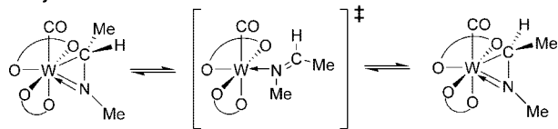
Scheme 4. Possible Mechanisms for Interconversion of Diastereomers in 3b
