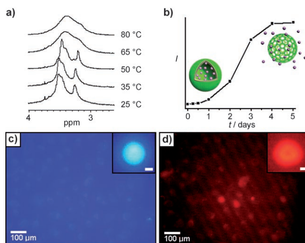
Figure 4. a) ^1\text{H} NMR spectra of ethylene oxide regions of 2 . b) Time course of calcein release from closed capsules of 2 . Fluorescence microscopy images of HeLa cells c) after intracellular delivery of the capsules and d) rhodamine-labeled DNA oligomer. Images of the capsules after DNA encapsulation showing that the blue fluorescence from the capsules (inset in c) overlaps with the red fluorescence from the DNA (inset in d). Scale bars in the insets: 4 \mu\text{m} .
