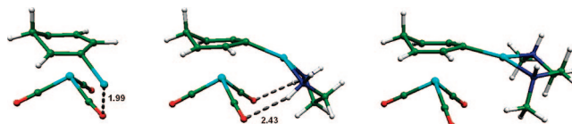
Figure 3. Representation of the lithiated species in position C 2 (left) and C 3 (center and right): Li + cation alone (left), Li + cation coordinated to L H-H (see text for notation, center), and the retained model of a Li + cation coordinated to L H-Me (right). Distances of the undesired interactions are given in Å.
