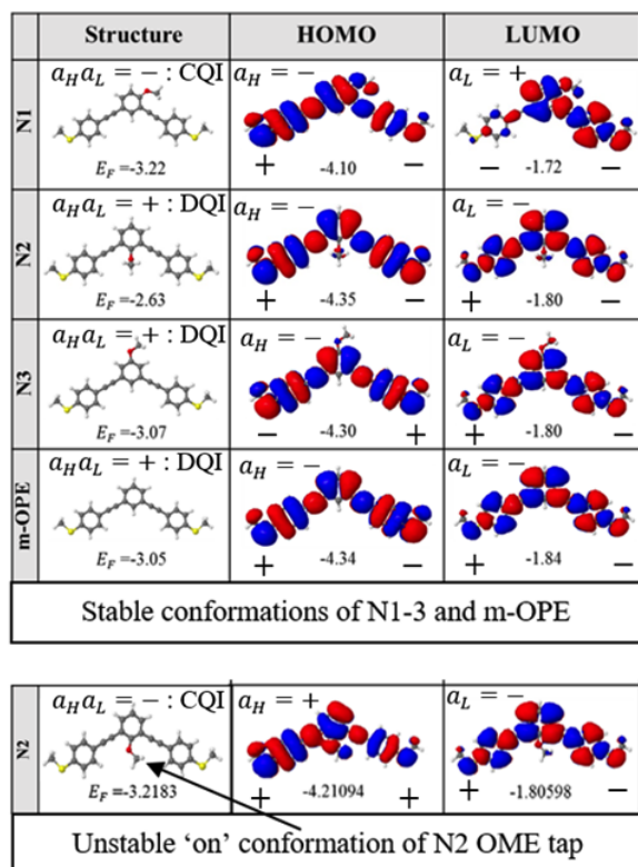
Figure 4. HOMOs and LUMOs of molecules N1-3 and the parent m -OPE. Blue regions are positive and red regions are negative. As an example, for N1 the HOMO at the left end of the molecule is positive (+) and at the right end it is negative (-). Therefore, since these have opposite signs, a_H is negative (-). Similarly for N1 , a_L is negative. Since the product of a_H a_L is positive (+), N1 will exhibit CQI.
