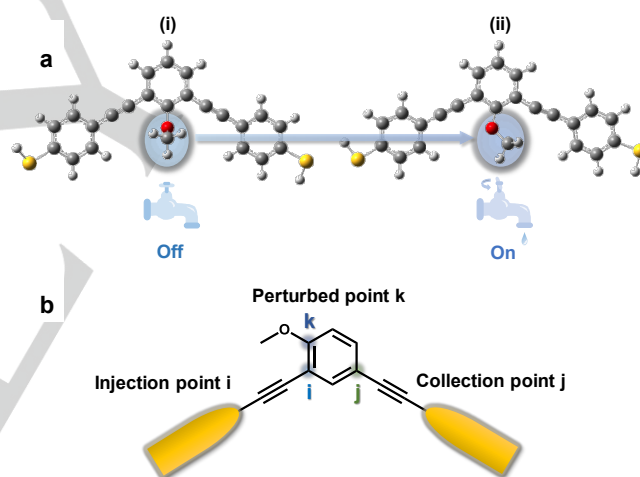
Figure 2. a) Two conformations of the molecular tap M2 (drawn as the free thiol). Rotating the OMe pendant group from the ‘off’ conformation (i) to the ‘on’ conformation (ii) switches the m -OPE molecule from low to high conductance as the position of the DQI feature shifts. b) A conceptual view of the magic ratio model of a molecular junction. The yellow regions represent compound electrodes, which inject and collect electrons via triple bonds into \pi -orbitals of the central ring at points i and j respectively. A perturbation associated with a pendant group is introduced at site k , illustrated schematically here for the substitution pattern of M1 / N1 .
