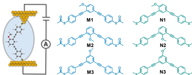
Figure 1. Schematic of STM-BJ setup and the chemical structures of the molecules investigated in this work.
