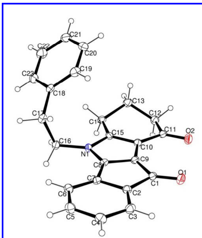
Figure 2. View of the crystal structure of 4c with our numbering scheme, displacement ellipsoids are drawn at the 30% probability level. Note: the numbering used here is specific to the crystallographic studies, and therefore different from that shown in Table 1 and used all along the text.
