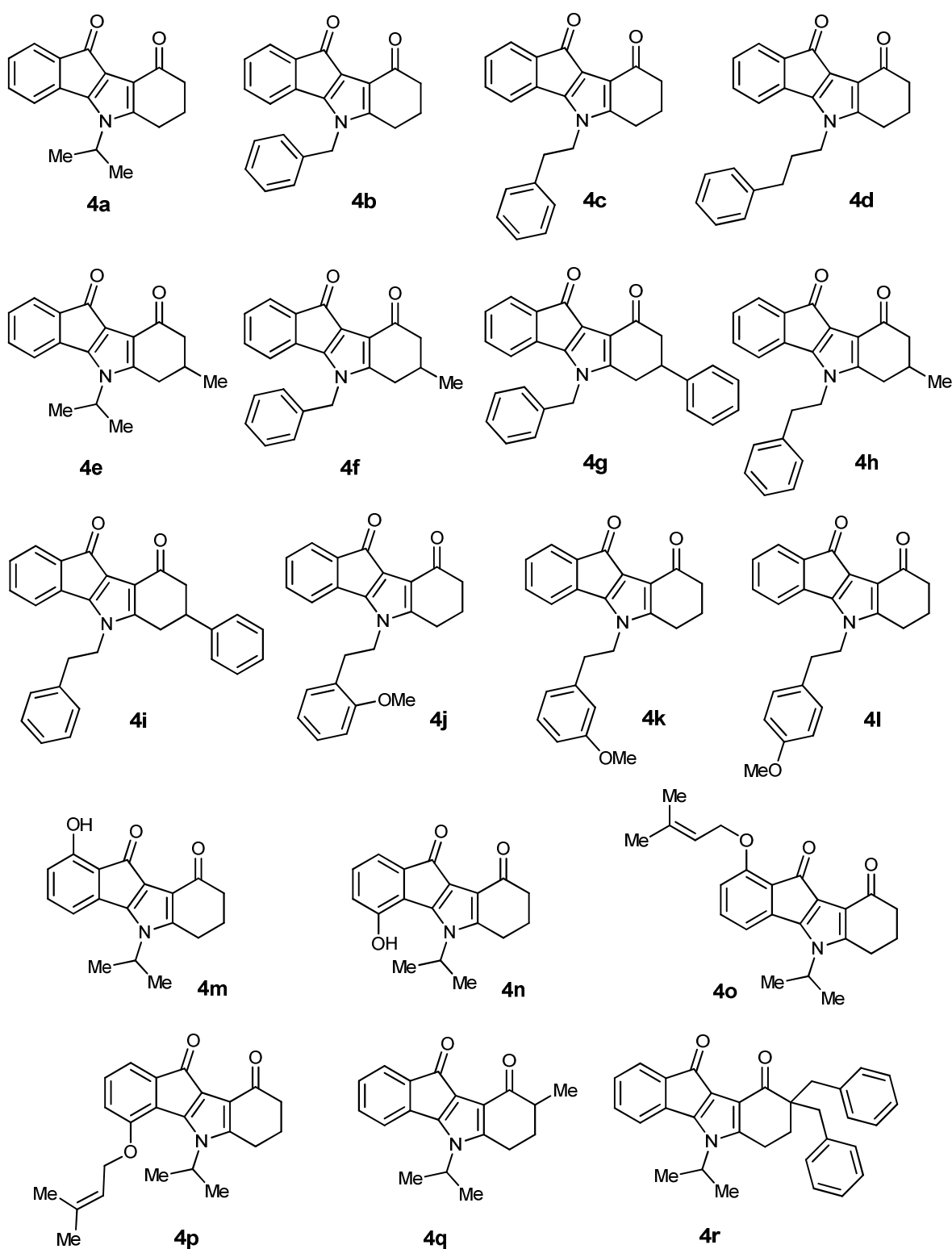
Figure 1. Substitution patterns of 4a-r . Note: compounds 4a-d and 4f-h are described in reference 33, and compound 4e in reference 37.
