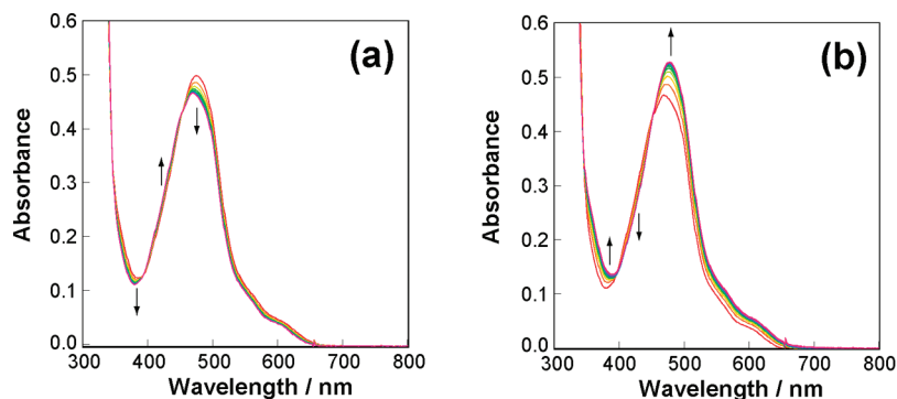
Figure 3. UV-vis absorption spectral changes of a THF solution (4 mL) containing Ru-DMF 2+ (0.051 mM) during irradiation using 436 nm light ( 0.23 \pm 0.02 \mu\text{einstein s}^{-1} ), recorded up to 3 min at intervals of 10 s (a) and recorded after stopping irradiation at intervals of 30 min (b).
