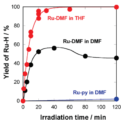
Figure 9. Formation yield of the \text{Ru-H}^+ versus irradiation time for the photochemical reactions of \text{Ru-DMF}^{2+} in THF (red), \text{Ru-DMF}^{2+} in DMF (black), and \text{Ru-py}^{2+} in DMF (blue). The solutions containing the complex (0.05 mM) and \text{NEt}_3 (2.0 M) were irradiated using 436 nm light ( 0.23 \pm 0.02 \mu\text{einstein s}^{-1} ) under an Ar atmosphere.
