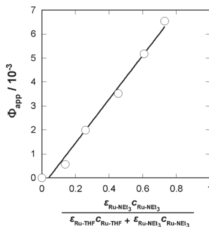
Figure 10. Dependence of the quantum yield of the formation of \text{Ru-H}^+ on the ratio of photons absorbed by \text{Ru-NEt}_3^{2+} to that by the equilibrium mixture of \text{Ru-THF}^{2+} and \text{Ru-NEt}_3^{2+} at 436 nm.
