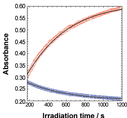
Figure 8. UV-vis absorption changes of a THF solution containing \text{Ru-DMF}^{2+} (0.051 mM) and \text{NEt}_3 (2 M) during irradiation with 436 nm light for 180–1200 s recorded with 5 s intervals, detected at 436 nm (blue circle) and 550 nm (red circle). The fitting curves were obtained using eqs 6 and 8.
