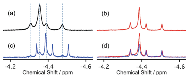
Figure 2. ^1\text{H} NMR analysis in \text{CDCl}_3 . (a) Initial sample of e\text{H}_2@2 . (b) After treatment of e\text{H}_2@2 to produce e\text{H}_2@3 . (c) After treatment of e\text{H}_2@3 with liquid \text{O}_2 at 77 K and sample workup. (d) Normalized overlap of (b) and (c). Dotted lines indicate the e\text{H}_2@2 signals.
