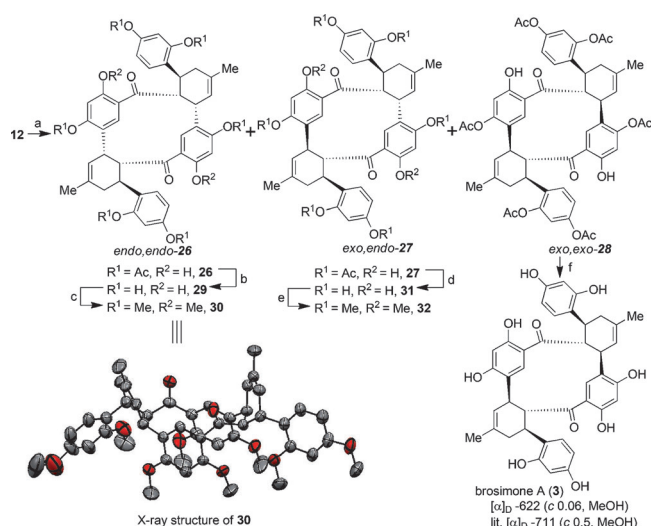
Scheme 5. a) (S)-VANOL, \text{BH}_3\cdot\text{THF} , \text{AcOH} , 5 Å M.S., THF, RT, 96 h, 61 % ( 26/27/28 = 28%:20%:13 %), 98 % ee for endo,endo - 26 , 95 % ee for exo,exo - 28 , recovered (S)-VANOL (91 %); b) \text{K}_2\text{CO}_3 , \text{MeOH}/\text{H}_2\text{O} (10:1), RT, 1.5 h, 75 %; c) \text{Me}_2\text{SO}_4 , \text{K}_2\text{CO}_3 , acetone, reflux, 16 h, 74 %, d) \text{K}_2\text{CO}_3 , \text{MeOH}/\text{H}_2\text{O} (10:1), RT, 1 h, 75 %; e) \text{MeI} , \text{K}_2\text{CO}_3 , acetone, reflux, 24 h, 63 %; f) \text{K}_2\text{CO}_3 , \text{MeOH}/\text{H}_2\text{O} (10:1), RT, 1 h, 70 %. Thermal ellipsoids shown at 50 % probability. [23]
