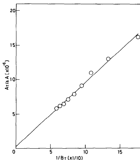
Fig. 3. Plot of A_T/\Delta A vs. 1/B_T for the coordination of diethylamine to \text{Cr(IV)O(TPP)} .
