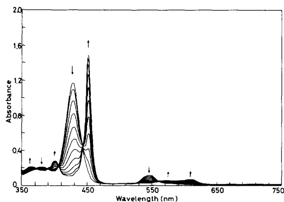
Fig. 2. Visible spectral changes occurring upon titration of a \text{Cr(IV)O(TPP)} solution with n -butylamine. Porphyrin concentration is 6.50 \times 10^{-5} M. Spectrum recorded at 25^\circ\text{C} with \text{CH}_2\text{Cl}_2 as the solvent. 20 \mu\text{l} of neat n -butylamine was successively added to 2 ml solution of \text{Cr(IV)O(TPP)} .
