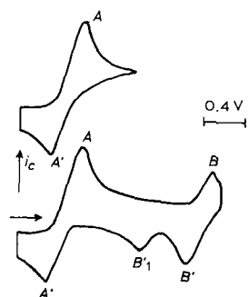
Fig. 3. Cyclic voltammogram at -30^{\circ}\text{C} of \text{V}^{\text{IV}}\text{LX}_2 in thf. Starting potential: +0.8\text{ V} ; sweep rate 200\text{ mV s}^{-1} .
