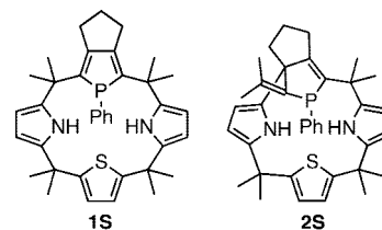
Chart 1. Structures of Phosphole-Containing Hybrid Calixpyrroles 1S and 2S
