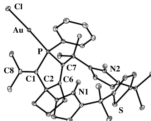
Figure 9. ORTEP diagram of 12 out (30% probability ellipsoids). Hydrogen atoms are omitted for clarity. Selected bond lengths (Å) and angles (deg): Au—Cl, 2.2871(4); Au—P, 2.2381(4); C1—C2, 1.532(2); C1—C8, 1.343(3); C2—C6, 1.529(3); C6—C7, 1.343(3); Cl—Au—P, 176.24(2).
