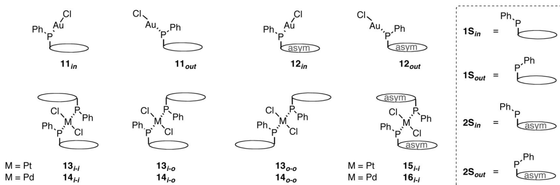
Figure 7. Simplified representations of the metal complexes.
