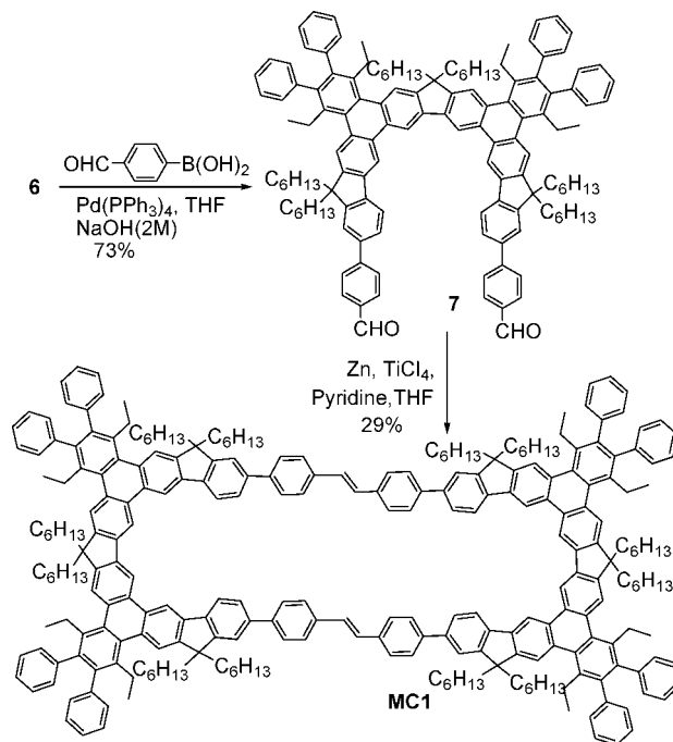
Scheme 2. Synthetic Route to MC1
