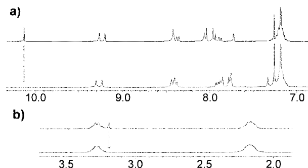
Figure 2. (a) 1 H NMR spectra of 7 (black) and MC1 (blue) from 7.0–11.0 ppm. (b) 1 H NMR spectra of 8 (black) and MC2 (blue) from 2.0–3.5 ppm.
