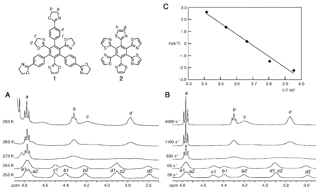
Figure 6. (A) Partial VT 1 H NMR spectra of [Ag 9 I 2 ·2 2 ] 9+ complex (500 MHz, CD 3 OD, [1] = [2] = 3.7 mM). (B) Simulated spectra of H a , H b , H c , and H d protons for various exchange rates. (C) Eyring plots.
