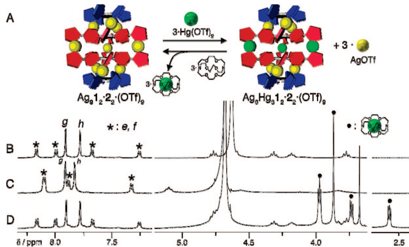
Figure 8. Interconversion between the \text{Ag}_9\text{L}_2\cdot 2\text{L}\cdot (\text{OTf})_9 and \text{Ag}_6\text{Hg}_3\text{L}_2\cdot 2\text{L}\cdot (\text{OTf})_{12} complexes. (A) Schematic representation of an interconversion between the \text{Ag}_9\text{L}_2\cdot 2\text{L}\cdot (\text{OTf})_9 and \text{Ag}_6\text{Hg}_3\text{L}_2\cdot 2\text{L}\cdot (\text{OTf})_{12} complexes. (B–D) ^1\text{H} NMR spectra for the replacement of the central three metal ions, \text{Ag}^+ \rightarrow \text{Hg}^{2+} \rightarrow \text{Ag}^+ (500 MHz, \text{CD}_3\text{OD} , 313 K, [\text{1}] = [\text{2}] = 7.5 mM). (B) \text{Ag}_9\text{L}_2\cdot 2\text{L}\cdot (\text{OTf})_9 . (C) Upon addition of \text{Hg}(\text{OTf})_2 (3 equiv) to the sample for panel B, \text{Ag}_6\text{Hg}_3\text{L}_2\cdot 2\text{L}\cdot (\text{OTf})_{12} complex was formed. (D) Upon addition of [2,2,2]-cryptand (3 equiv) to the sample for panel C, \text{Ag}_9\text{L}_2\cdot 2\text{L}\cdot (\text{OTf})_9 complex was regenerated as a result of the formation of \text{Hg}^{2+} \subset [2,2,2]\text{-cryptand} .
