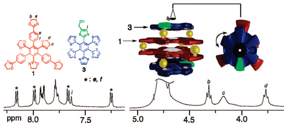
Figure 4. Partial VT ^1\text{H} NMR spectrum (500 MHz, \text{CD}_3\text{OD} ) of \text{Ag}_9\text{I}_2\cdot 32\cdot (\text{OTf})_9 ( [\text{Ag}_9\text{I}_2\cdot 32\cdot (\text{OTf})_9] = 4.0 mM, 303 K).
