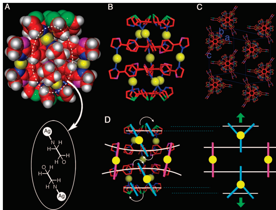
Figure 3. Crystal structure of the \text{Ag}_9\text{I}_2\cdot 22\cdot (\text{OTf})_9 complex. (A) A space filling model. (B) A cylinder model. Hydrogen atoms are omitted for clarity. Color labels: red, carbon; yellow, silver; blue, nitrogen; purple, oxygen; green, sulfur. (C) A packing diagram of [\text{Ag}_9\text{I}_2\cdot 22]^{9+} viewed from a rotation axis of the complex. Hydrogen atoms and counteranions are omitted for clarity. (D) Schematic depiction of the proposed ground and transition geometries of the ligand exchange processes taking place in the [\text{Ag}_9\text{I}_2\cdot 22]^{9+} complex.
