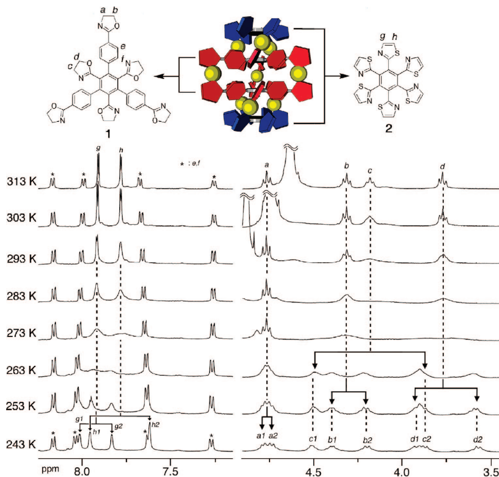
Figure 2. Partial VT ^1\text{H} NMR spectra (500 MHz, \text{CD}_3\text{OD} ) of a molecular rotor–transmitter–rotor, \text{Ag}_9\text{L}_2\cdot 2_2\cdot (\text{OTf})_9 . [\text{Ag}_9\text{L}_2\cdot 2_2\cdot (\text{OTf})_9] = 3.7 mM.
