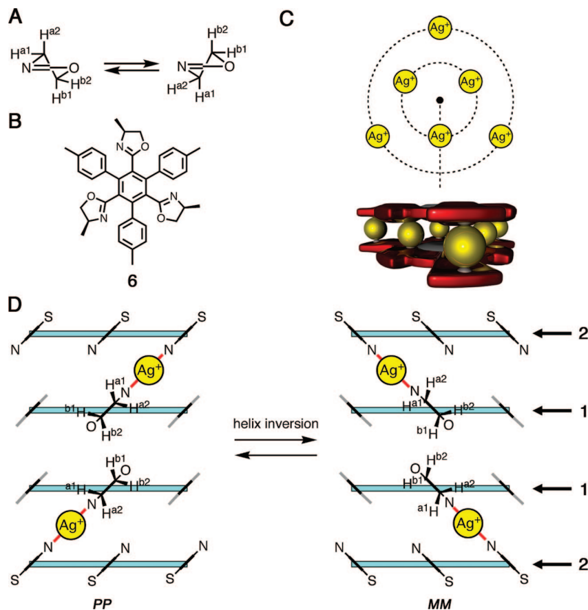
Figure 5. (A) Ring flip of an oxazoline ring between two twisted-boat conformations. (B) Chemical structure of asymmetric tris-monodentate ligand 6 . VT NMR spectra of [Ag 3 2· 6 ] 3+ were reported in ref 17. (C) Schematic representation of [Ag 6 I 2 ] 6+ complex. The synthesis and structural characterization of the complex were reported in ref 19. (D) Schematic representation of the helix inversion in [Ag 6 M 3 I 2 ·2 2 ] (3n+6)+ complexes (M n+ = Ag + or Hg 2+ ). PP and MM denote screw senses of the two molecular ball bearing moieties ([Ag 3 1·2] 3+ ) in their structures.
