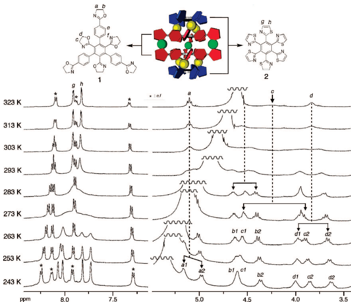
Figure 7. Partial VT ^1\text{H} NMR spectra (500 MHz, \text{CD}_3\text{OD} ) of a molecular rotor–transmitter–rotor, \text{Ag}_6\text{Hg}_3\text{L}_2\cdot 2\text{L}\cdot (\text{OTf})_{12} . [\text{Ag}_6\text{Hg}_3\text{L}_2\cdot 2\text{L}\cdot (\text{OTf})_{12}] = 3.7 mM.
