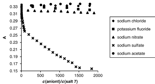
Fig. 2 Selectivity study of salt 7 for simple anions. Concentration of 7 = 2.2 \times 10^{-6} M in a solution of 68% \text{H}_2\text{O} -30% MeOH-2% DMSO, pH = 5.53, medium = 1 mM phosphate buffer, wavelength = 663 nm.
