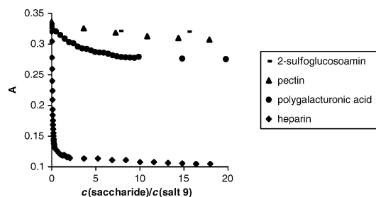
Fig. 4 Titration curves of the salt 9 with acid saccharides. Concentration of the salt 9 = 4.6 \times 10^{-6} M in a solution of 85% \text{H}_2\text{O} -15% PEG ( n = 9 ), pH = 5.53, 1 mM phosphate buffer, wavelength = 663 nm.
