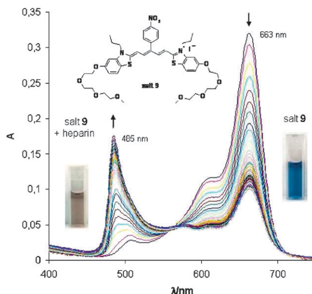
Fig. 3 Titration of 9 ( c = 4.6 \times 10^{-6} M) with heparin in a solution of 85% \text{H}_2\text{O} -15% PEG ( n = 9 ), 1 mM phosphate buffer pH = 5.53; no. of equivalents are from 0 to 100.
