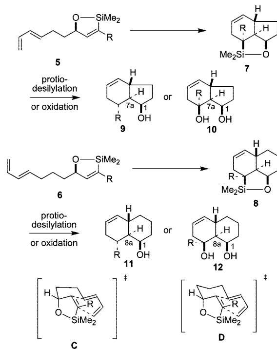
Scheme 2. Strategy for Intramolecular Diels–Alder Cyclizations of Siloxacyclopentene-Constrained Trienes 5 and 6
