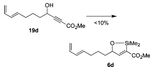
Scheme 5. Attempted Hydrosilylation of 19d
