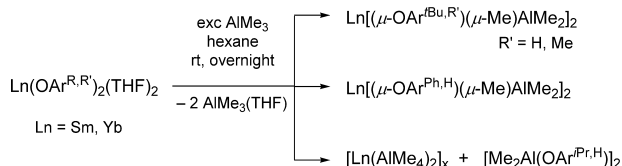
Scheme 1. TMA Adduct Formation versus Peralkylation of Lanthanide(II) Aryloxides with Excess of Trimethylaluminum 17
