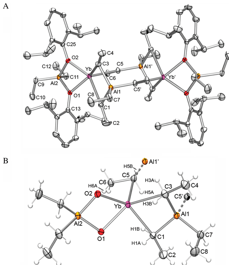
Figure 6. (A) Molecular structure of 9 with atomic displacement parameters set at the 50% probability level; hydrogen atoms are omitted for clarity. (B) \text{Yb}^{\text{II}} coordination environment in 9 emphasizing the agostically interacting hydrogen atoms (atomic displacement parameters set at the 50% probability level).
