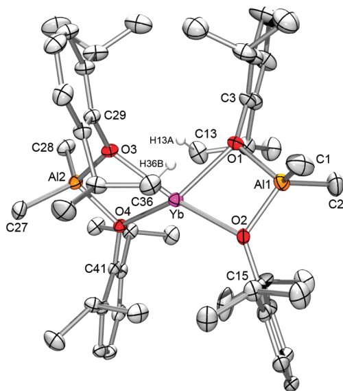
Figure 4. Molecular structure of 7b . Atomic displacement parameters are set at the 50% probability level and hydrogen atoms are omitted for clarity, except for agostically interacting H36B and H13A.
