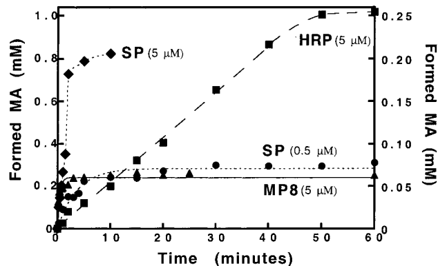
Figure 4. Operational stability of purified SP ( \cdots ) (left Y-axis), HRP ( --- ) (right Y-axis), and MP8 ( — ) (right Y-axis) in the conversion of MNMA (SP at 70^\circ C and pH 4; HRP and MP8 at 37^\circ C and pH 7.6). The enzyme concentration was 5 \mu M in all cases. As the MNMA conversion by 5 \mu M SP was hampered by substrate limitation, the operational stability of SP was determined also with 0.5 \mu M SP ( \bullet ) (right Y-axis).
