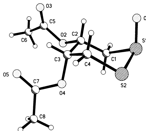
Fig. 1. Molecular structure of 3 in the crystal.
