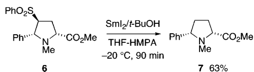
Scheme 1. Desulfonylation of 6
