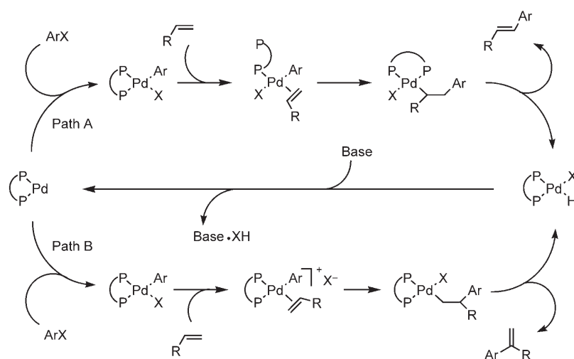
Scheme 2. The suggested neutral and cationic pathways of the Heck reaction.
