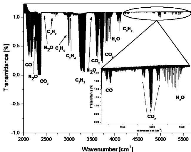
Figure 2. The FTIR absorption spectrum of the CO-N 2 -H 2 O mixture exposed to ten laser sparks and then trapped in liquid nitrogen.
