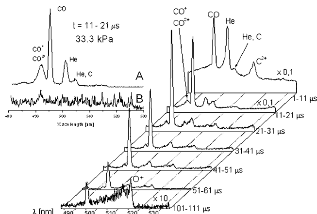
Figure 10. Time-resolved OES spectra of LIDB in the He–CO mixture (100:1) at a total pressure of 33.3 kPa.
