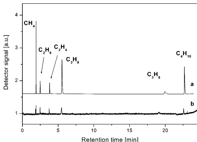
Figure 8. Comparison of gas chromatograms (FID signal) taken for (a) a mixture of standard hydrocarbons and (b) the CO–N 2 –H 2 O mixture trapped in liquid nitrogen after its exposure to ten laser shots.
