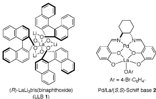
Figure 1. Structure of ( R )-LaLi 3 tris(binaphthoxide) ( 1 : LLB) and proposed structure of a Pd:La:( S,S )-Schiff base:OAr = 1:1:1:1 complex 2 .
