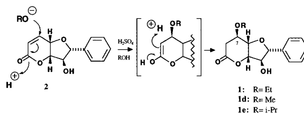
Figure 3. Preparation of (–)-etharvensin ( 1 ) and 7-alkoxy-furanopyrones ( 1d , 1e ) from (+)-altholactone ( 2 ).
