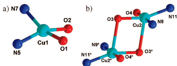
Figure 2. (a) Coordination environment around the terminal atom Cu1. (b) Coordination environment around the central atoms Cu2 and Cu2*. Selected bond distances (Å) around Cu1 and Cu2: Cu1–O2 1.882(5); Cu1–N5 1.927(5); Cu1–O1 1.928(4); Cu1–N7 2.016(5); Cu2–O4 1.915(4); Cu2–N9 1.958(5); Cu2–O3 1.974(4); Cu2–N11 1.985(5); Cu2–O3* 2.553(5). Important bond angles (deg) around Cu1 and Cu2: O2–Cu1–N5 156.3(2); O2–Cu1–O1 89.6(2); N5–Cu1–O1 92.2(2); O2–Cu1–N7 94.2(2); N5–Cu1–N7 93.0(2); O1–Cu1–N7 157.79(19); O4–Cu2–N9 177.18(18); O4–Cu2–O3 88.69(19); N9–Cu2–O3 90.9(2); O4–Cu2–N11 90.8(2); N9–Cu2–N11 90.5(2); O3–Cu2–N11 160.65(18); N9–Cu2–O3* 89.01(2); N11–Cu2–O3* 116.37(2); O4–Cu2–O3* 88.17(2); O3–Cu2–O3* 82.94(2).
