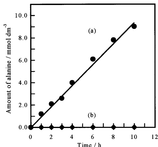
Figure 2. Production of D-alanine (a) and L-alanine (b) by electrochemical reduction at -0.7 V vs. Ag/AgCl of 0.1 \text{ mol dm}^{-3} phosphate buffer (pH 6.5, 20 ml) containing 30 \text{ mmol dm}^{-3} pyruvic acid and 30 \text{ mmol dm}^{-3} \text{NH}_4\text{OH} with the use of D-AOx/ADPy/GC electrode.
