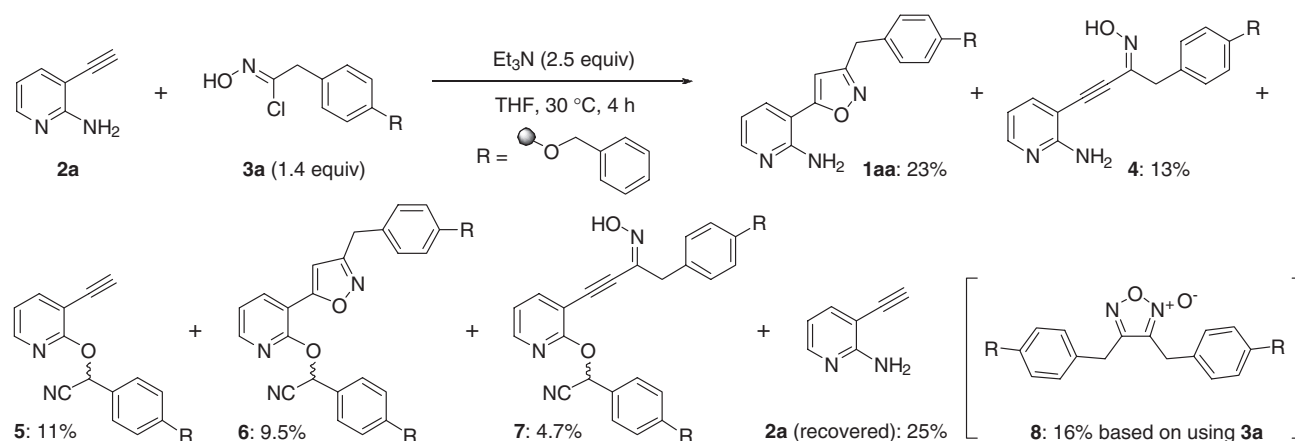
Scheme 1. Isolated products in the isoxazole synthesis without \text{ZnCl}_2 .
