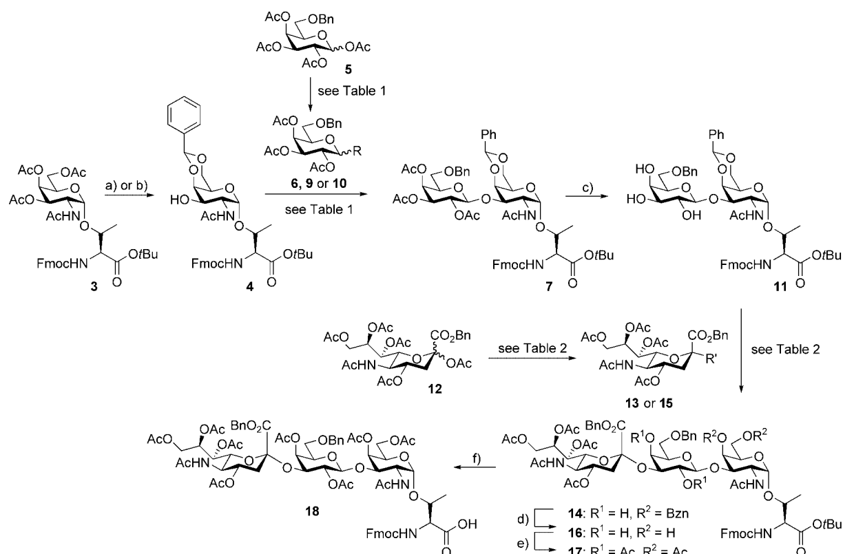
Scheme 2. Reagents and conditions: a) i) MeOH, NaOMe, pH 8.5, 3 h; ii) DMF, \alpha,\alpha -dimethoxytoluene, PTSA, 15 mbar, 50°C, 2 h, 44 %. b) i) MeOH, NaOMe, pH 8.5, 3 h; ii) MeCN, \alpha,\alpha -dimethoxytoluene, PTSA, room temperature, 15 h, 75 %. c) MeOH, NaOMe, pH 8.5, 12 h, 62 %. d) AcOH (80 %), 80°C, 1 h, 82 %. e) pyridine/Ac 2 O (2.3:1), DMAP, 6 h, 87 %. f) TFA, anisole, quant. DMAP = N,N -dimethylaminopyridine; DMF = dimethylformamide; DTBP = di- tert -butylpyridine; PTSA = p -toluenesulfonic acid; TFA = trifluoroacetic acid.
