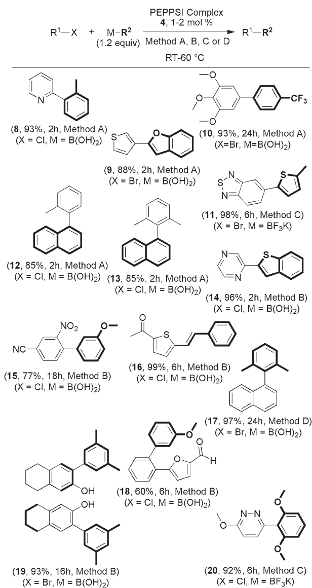
Scheme 3. \text{Sp}^2\text{--}\text{sp}^2 substrate scope. All reactions were performed by using standard laboratory techniques. Method A: 4 (1 mol %), \text{KtOBu} (1.3 equiv), reagent grade isopropanol, RT. Method B: 4 (2 mol %), dioxane, 60 °C. Method C: 4 (2 mol %), \text{K}_2\text{CO}_3 (3.0 equiv), methanol, 60 °C. Method D: 4 (2 mol %), \text{KOH} (3.0 equiv), dioxane, RT. Compound 11 was isolated in 70% yield after 12 h at RT. Compound 19 was prepared from 4 (4 mol %) \text{K}_2\text{CO}_3 (6.0 equiv), and \text{RB(OH)}_2 (2.4 equiv); this product has been made on a 10 g scale with a yield of 80%.
