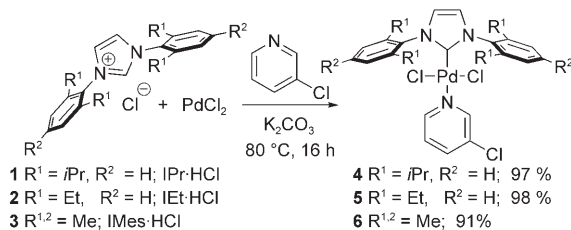
Scheme 1. Synthesis of NHC-PdCl 2 -3-chloropyridine complexes.
