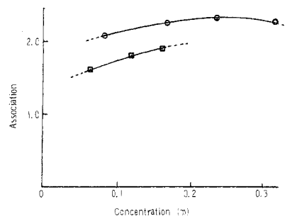
Figure 2. Association of potassium di- sec -butylhydridomagnesium (a) and potassium di- n -butylhydridomagnesium (o) in benzene.
