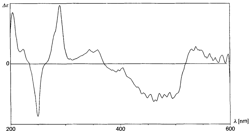
Fig. 4. CD Spectrum of ( all-E ,2S,2'S)- 15 at +25^\circ
