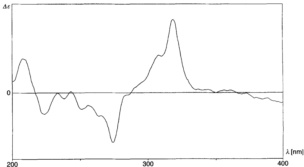
Fig. 2. CD Spectrum of (all-E,2S,2'S)-2 at +20^\circ
