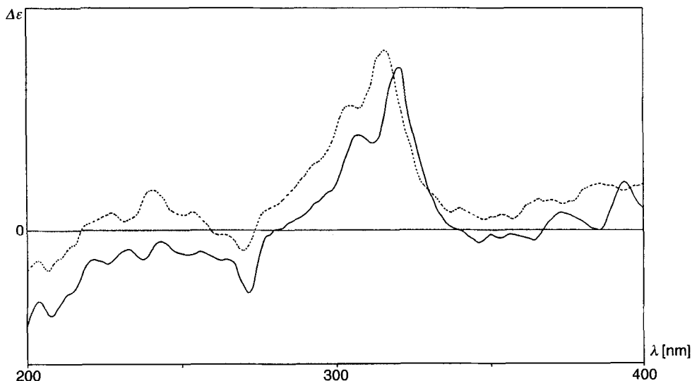
Fig. 1. CD Spectra of (all-E,2S,2'S)-1 (— -180^\circ , --- +20^\circ )
