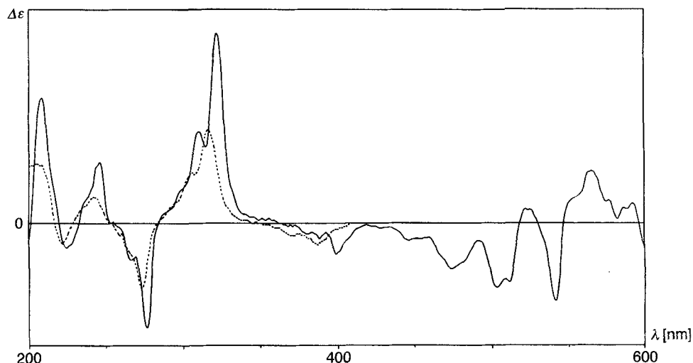
Fig. 3. CD Spectra of ( all-E ,2S,2'S)- 3 (— -180^\circ , --- +20^\circ )
