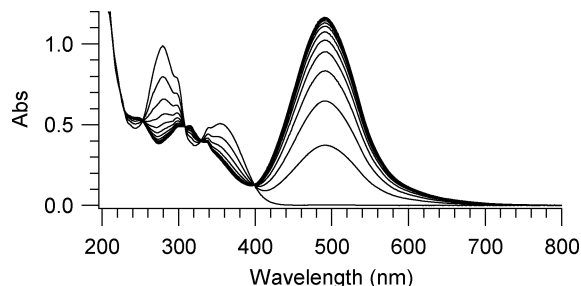
Figure 2. Irradiation of DHA 20a ( 1.2 \times 10^{-5} M) in MeCN with light (354 nm) during 0–140 s (10-s steps). The final VHF ( 20b ) absorption spectrum is indicated by the thick curve.
