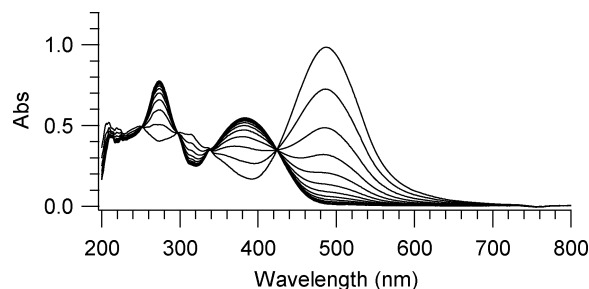
Figure 3. Thermal back-reaction of VHF 20b ( 1.2 \times 10^{-5} M) in MeCN monitored at 70 °C (2-min steps). The final DHA ( 20a/26a ) absorption spectrum is indicated by the thick curve.
