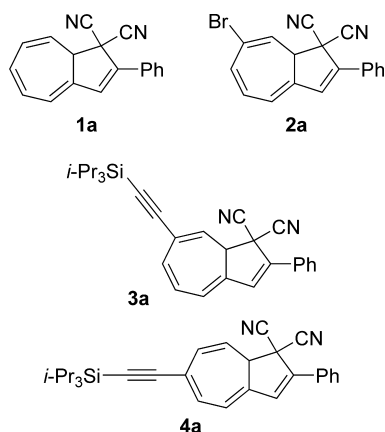
Chart 1. Functionalized DHAs
