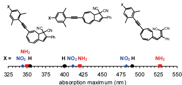
Figure 5. Summary of absorption maxima for the aryl-substituted DHAs and VFHs. The shoulder at ca. 350 nm was plotted for 21a .
