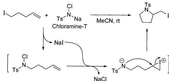
Scheme 1. A Representative Example of Previous Studies on the Synthesis of a Pyrrolidine
