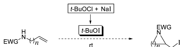
Scheme 2. Proposed Cyclization of N -Alkenylamides with t -BuOI
