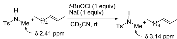
Scheme 3. Iodination Reaction: Sulfonamide versus Olefin
