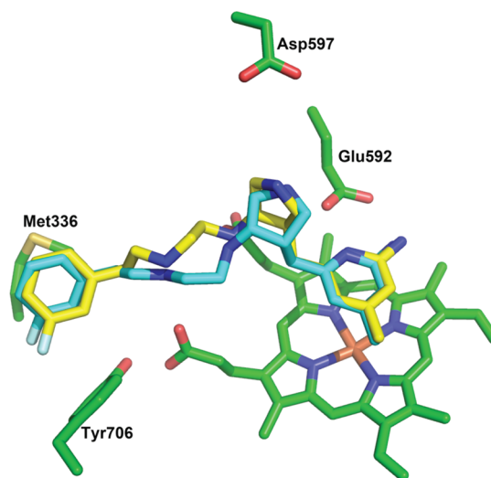
Figure 3. (3′ R ,4′ R )-2 (yellow) modeled in the same orientation as (3′ S ,4′ S )-2 (cyan) with an emphasis placed on minimizing steric clashes. It is not possible to model (3′ R ,4′ R )-2 in the (3′ S ,4′ S )-2 orientation and still maintain optimal inhibitor–protein H-bonds and minimal steric clashes.
