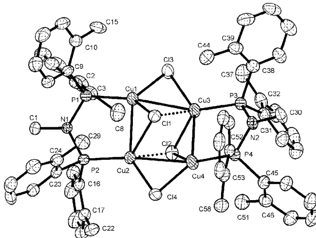
Figure 6. Crystal structure of [(Ar 2 PN(Me)PAR 2 )Cu 2 Cl 2 ] 2 {Ar = 2-C 6 H 4 (Me)} ( 23 ) (hydrogens and solvent omitted for clarity).
