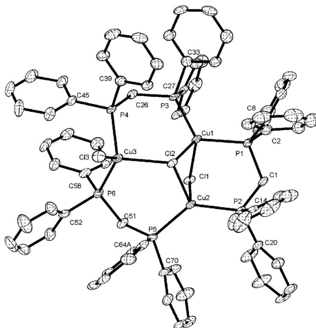
Figure 2. Crystal structure of [(\text{Ph}_2\text{PCH}_2\text{PPh}_2)\text{CuCl}]_3 ( 13 ). Hydrogens and solvent are omitted for clarity.
