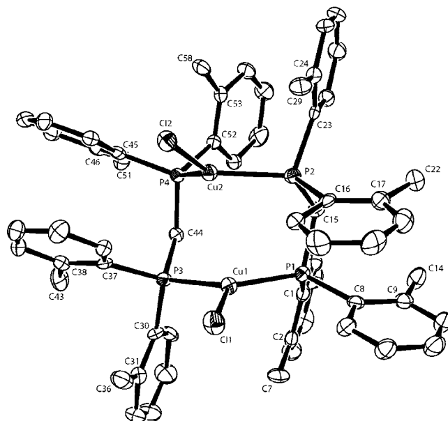
Figure 4. Crystal structure of [(Ar 2 PCH 2 PAR 2 )CuCl] 2 {Ar = 2-C 6 H 4 (Me)} ( 14 ) (hydrogens and solvent omitted for clarity).
