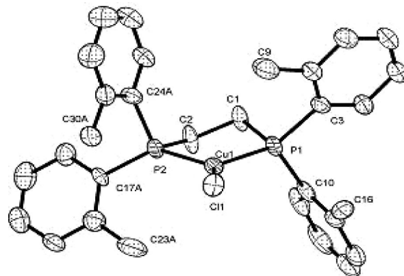
Figure 5. Crystal structure of [(Ar 2 PCH 2 CH 2 PAR 2 )CuCl] {Ar = 2-C 6 H 4 (Me)} ( 17 ) (hydrogens omitted for clarity).
