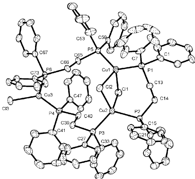
Figure 3. Crystal structure of [(Ph 2 PCH 2 CH 2 PPh 2 )CuCl] 3 ( 16 ) (hydrogens omitted for clarity).
