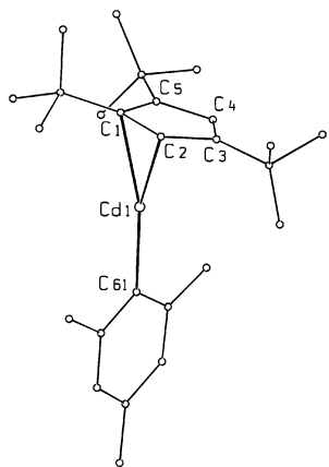
Figure 3. Line drawing of mesityl(tetraoisopropylcyclopentadienyl)-cadmium ( 3 ).
