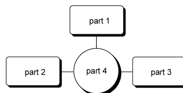
Fig. 1. The Four Parts of an Active KSP Inhibitor in Our Model (Part 1: Aromatic Ring; Part 2: Hydrophobic Group; Part 3: Side Chain; Part 4: Flexible Heterocyclic Ring)
