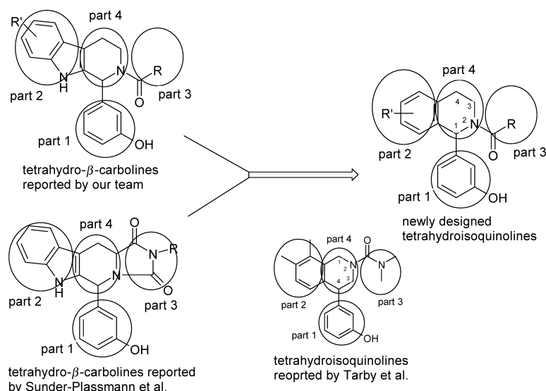
Fig. 3. Tetrahydroisoquinoline 1s Selected as the Core of New KSP Inhibitors
