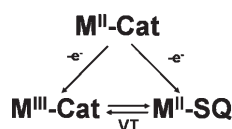
Scheme 1. Thermodynamical processes involved in VT equilibrium.
