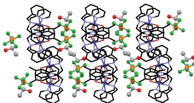
Figure 4. View of the packing of 1 along the (101) direction, thus demonstrating the alternating layers of the cationic molecules and the PF 6 − and solvent molecules.
