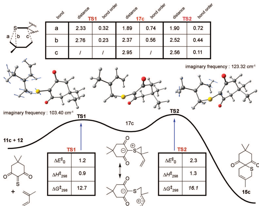
FIGURE 6. Calculated B3LYP/6-31+G(f2d) free energy profiles computed at 25 °C for the reaction of thione 11c with isoprene 12 leading to major product 15c via thiiranium zwitterion intermediate 17c . Bond distances (Å), bond orders, and relative energies (kcal/mol) are shown for the TSs. The value of the only imaginary frequency of each TS is indicated together with a vectorial description of atomic motions.
