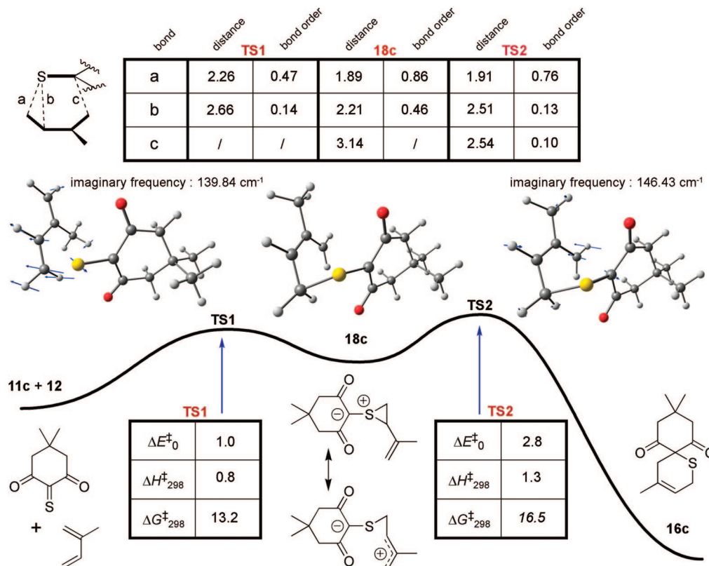
FIGURE 7. Calculated B3LYP/6-31+G(f2d) free energy profiles computed at 25 °C for the reaction of thione 11c with isoprene 12 leading to minor product 16c via thiuranium zwitterion intermediate 18c . Bond distances (Å), bond orders, and relative energies (kcal/mol) are shown for the TSs. The value of the only imaginary frequency of each TS is indicated together with a vectorial description of atomic motions.
