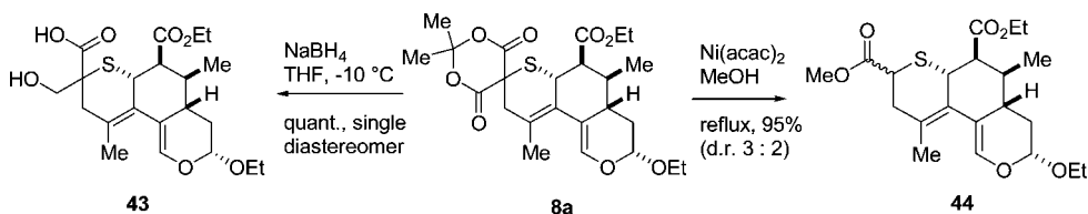
SCHEME 8. Mild Conditions for the Cleavage of the Dioxanedione Moiety
