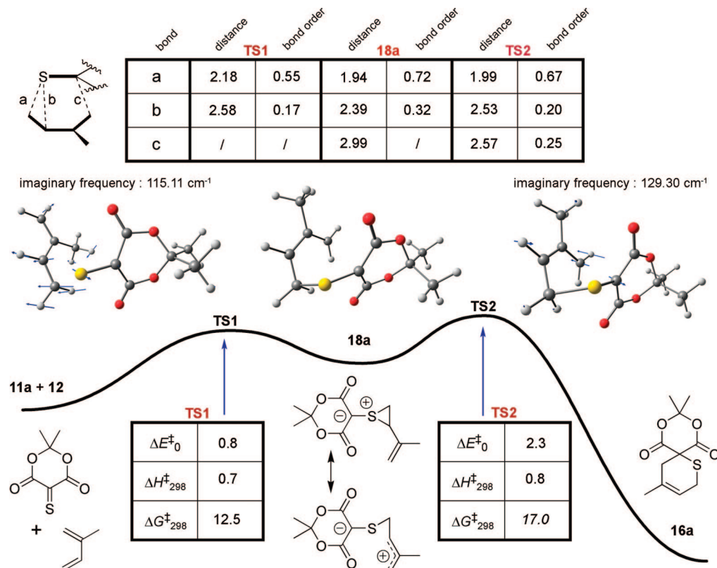
FIGURE 5. Calculated B3LYP/6-31+G(f2d) free energy profiles computed at 25 °C for the reaction of thione 11a with isoprene 12 leading to minor product 16a via thiiranium zwitterion intermediate 18a . Bond distances (Å), bond orders and relative energies (kcal/mol) are shown for the TSs. The value of the only imaginary frequency of each TS is indicated together with a vectorial description of atomic motions.
